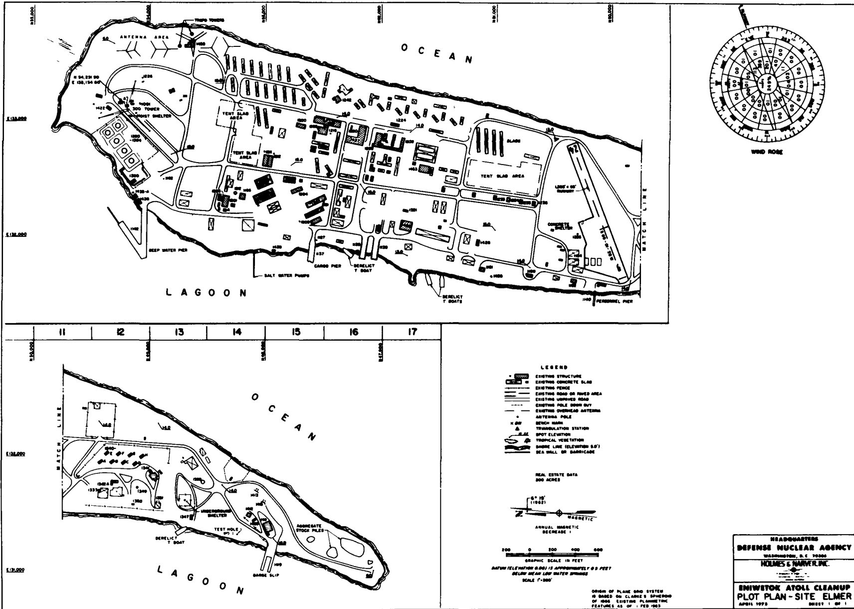
FIGURE 141. SITE ELMER, PLOT PLAN
